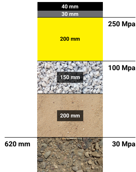
2. StabilRoad® highway
