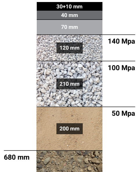
1. Traditional highway
