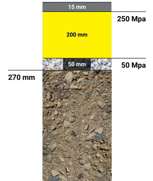
4. StabilRoad® vallatee
